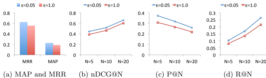
Fig. 2: The performance of item recommendations on the Movielens dataset with \epsilon = 0.05 and \epsilon = 1.0 using CoFM R .
